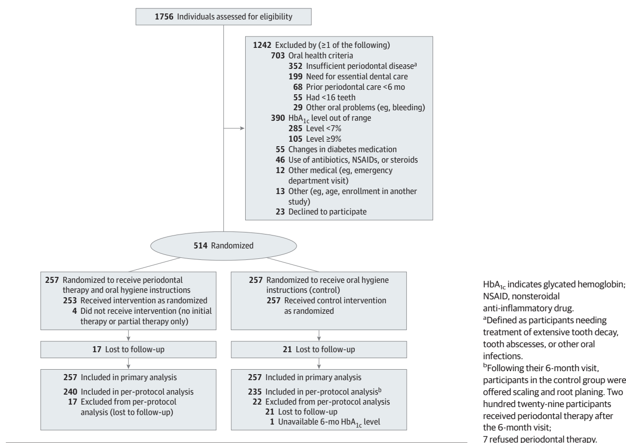
Figure 1. Study Flow
